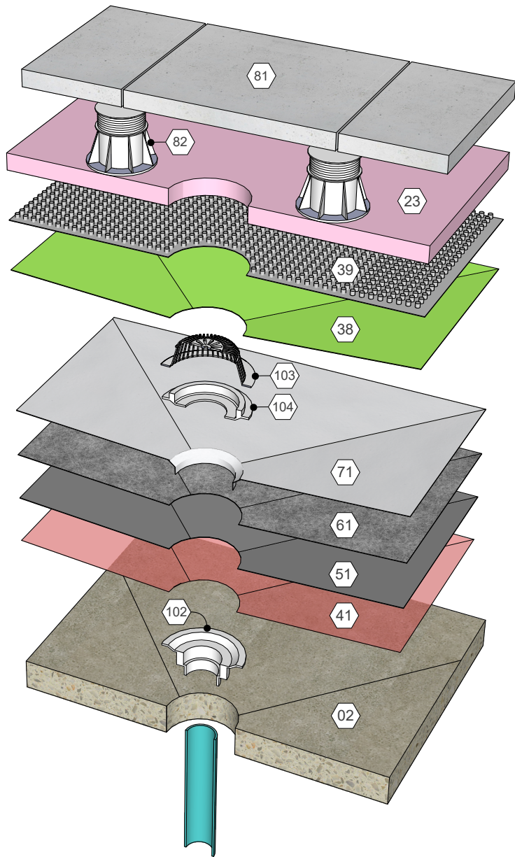
AlphaGuard® MT/MTS Roof Drain Detail, Direct to Concrete Detail 10221
